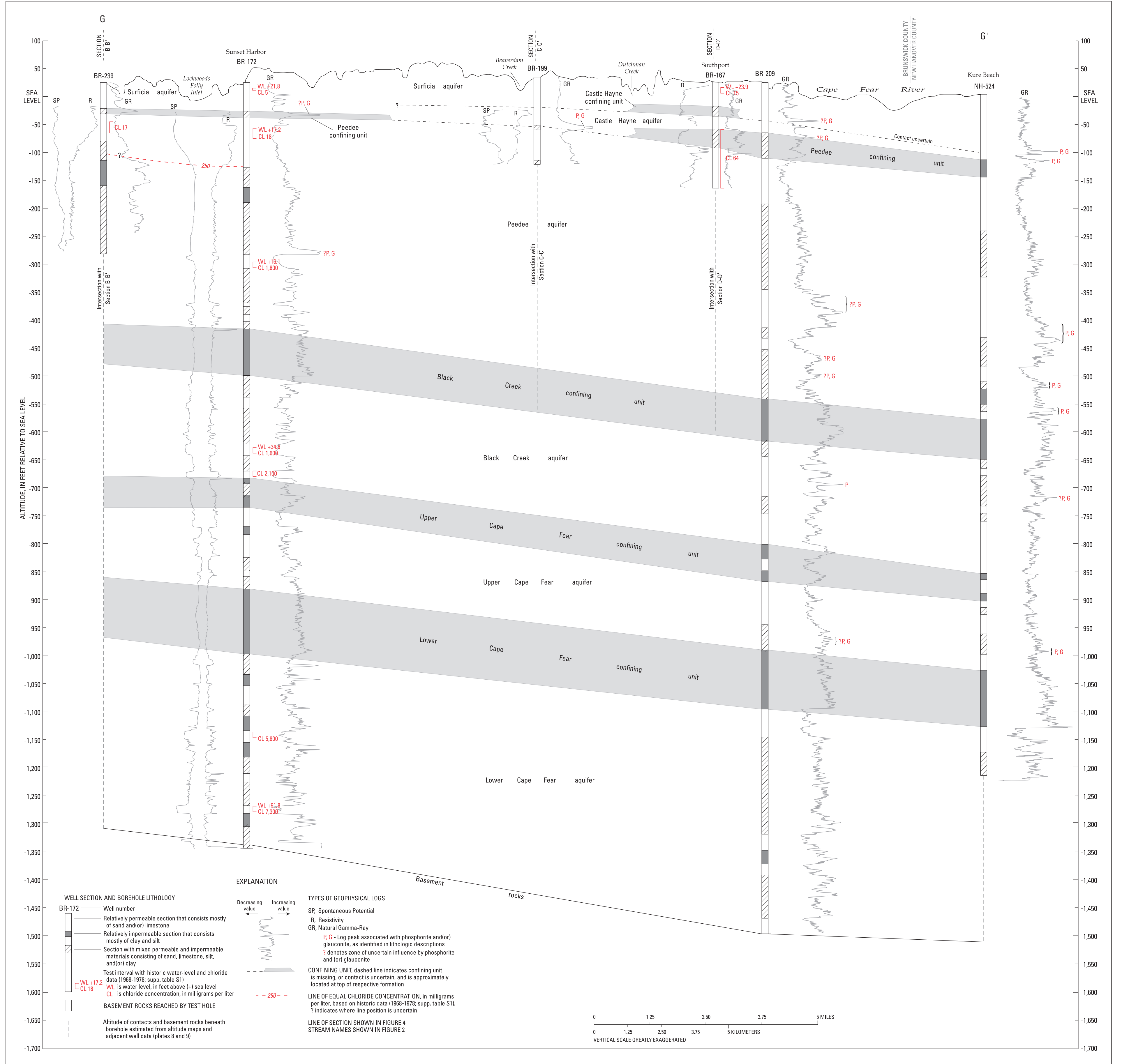
Plate 7. HYDROGEOLOGIC SECTION G-G', BRUNSWICK COUNTY, NORTH CAROLINA
