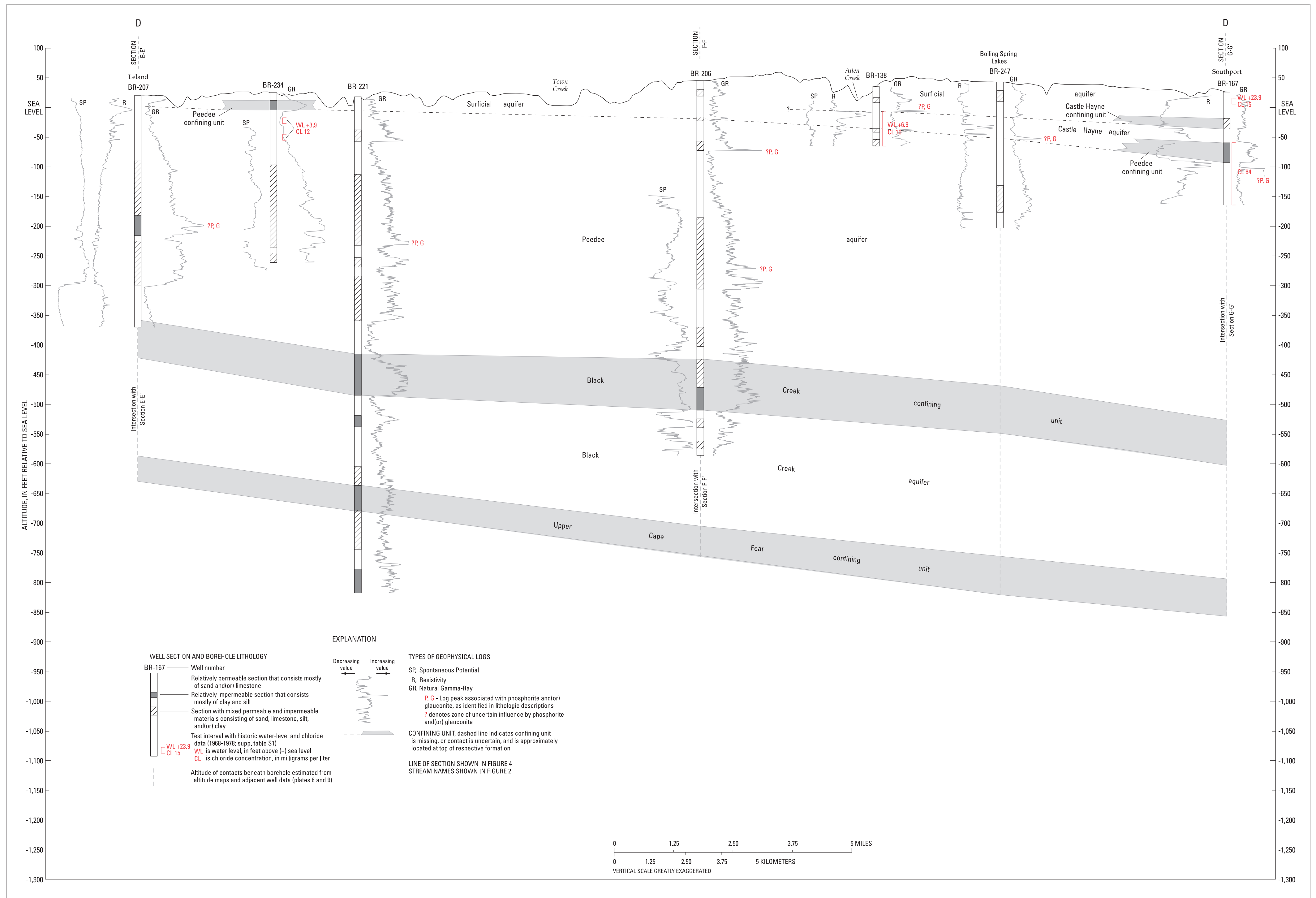
Plate 4. HYDROGEOLOGIC SECTION D-D', BRUNSWICK COUNTY, NORTH CAROLINA
